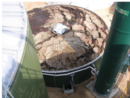
Defect at the foil cap → switch off of agitator → formation of 1.5m swim layer
