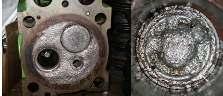
Damage at gas engine – demolition of valvet
